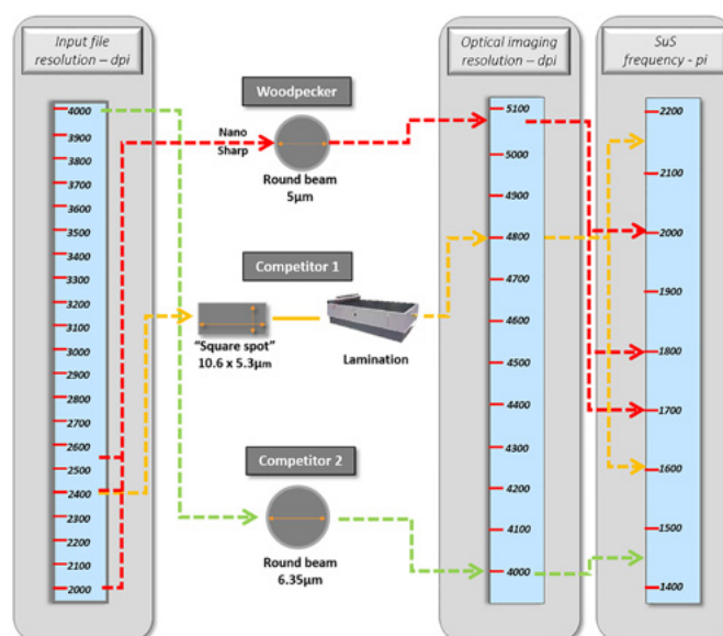
Half-tone Line Screen Dots lines per inch LPI SuS spatial frequency per inch PI
